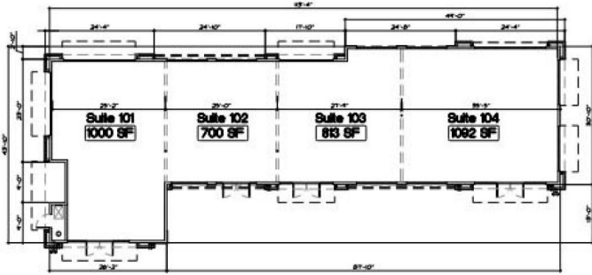
BUILDING #1 3,605 s.f.
